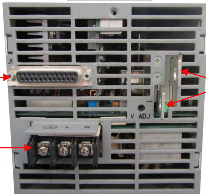
IO Connections
